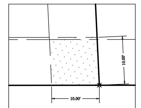
DETAIL "A" TYP. 10' X 10' SIGN EASEMENT
